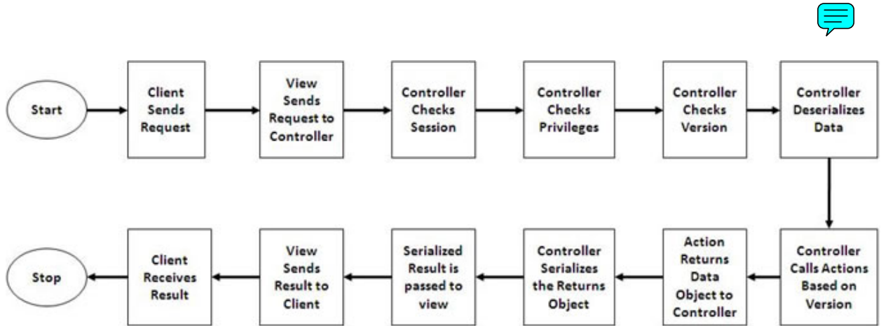
Figure 3.14. Flow diagram used in planning for the development from data store to web service interaction.
